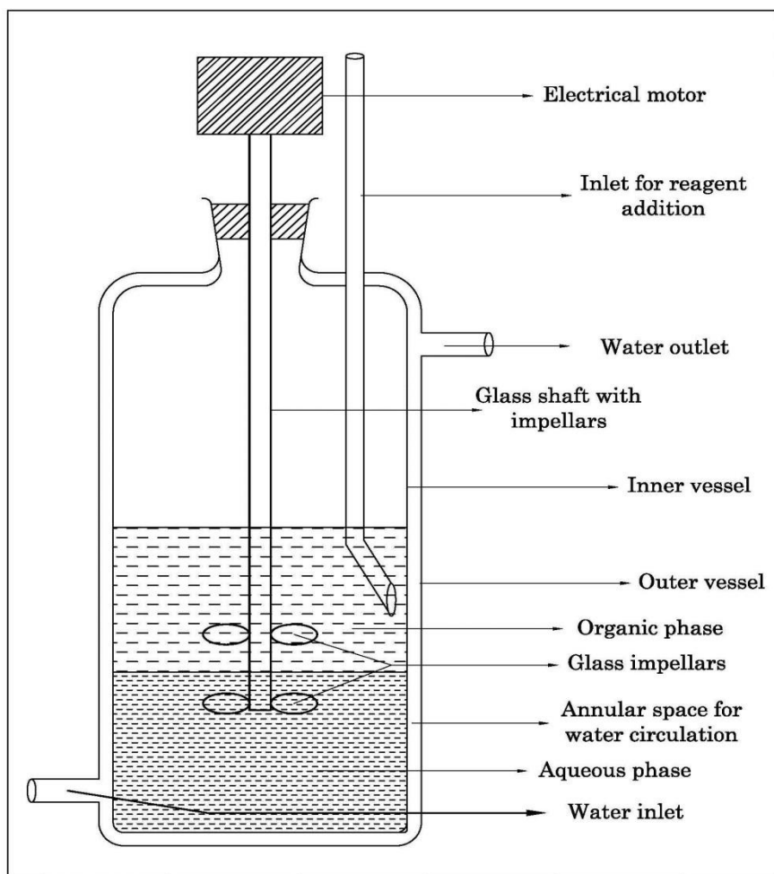
Fig.1 Schematic diagram of Lewis cell
