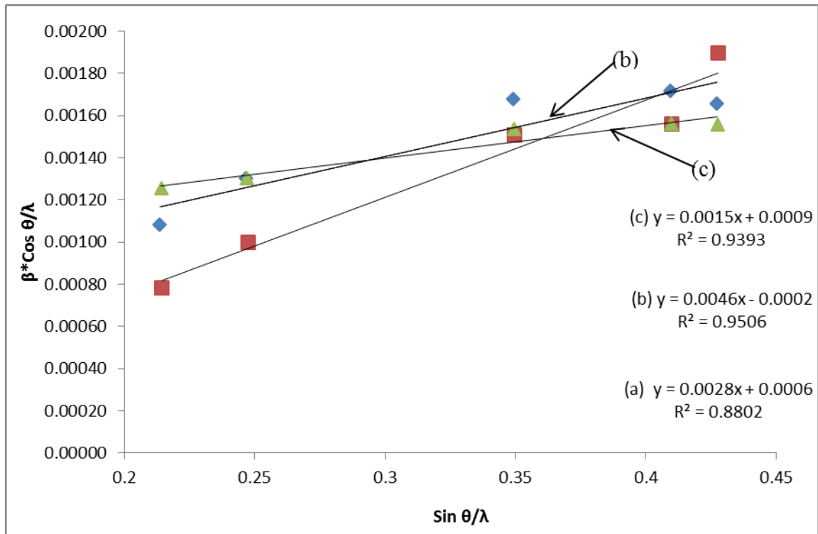
Fig.2: \beta^* \cos \theta / \lambda vs \sin \theta / \lambda plots: (a) Al-5vol.%Al 2 O 3 nanocomposite powder produced by HEMM; (b) Al-5vol.%Al 2 O 3 nanocomposite disk produced by powder compact forging; (c) Al-5vol.%Al 2 O 3 nanocomposite rod produced by powder compact extrusion.
